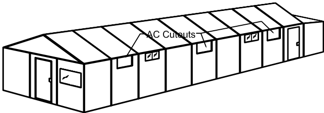
12' x 37' Dormitory Unit with 12' x 4' Shower and Toilet Room
